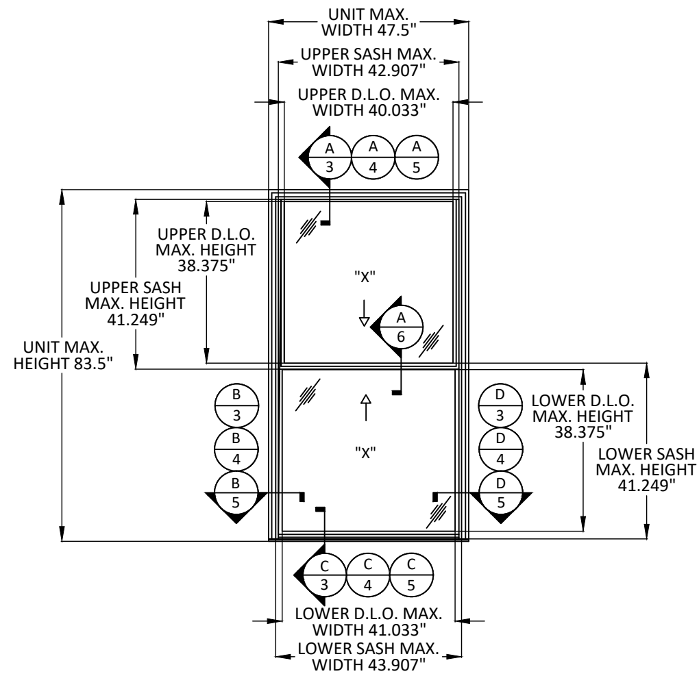
TYPICAL ELEVATION DOUBLE HUNG EQUAL
