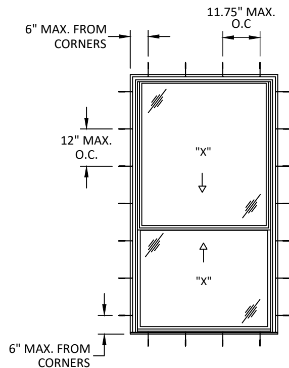
ANCHOR LAYOUT THROUGH FRAME INSTALLATION (EQUAL OR ORIEL)
