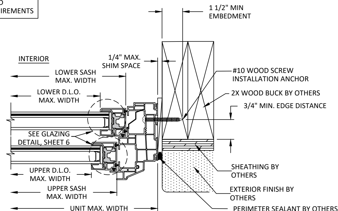
D 4 HORIZONTAL SECTION THROUGH FRAME INSTALLATION WOOD BUCK
