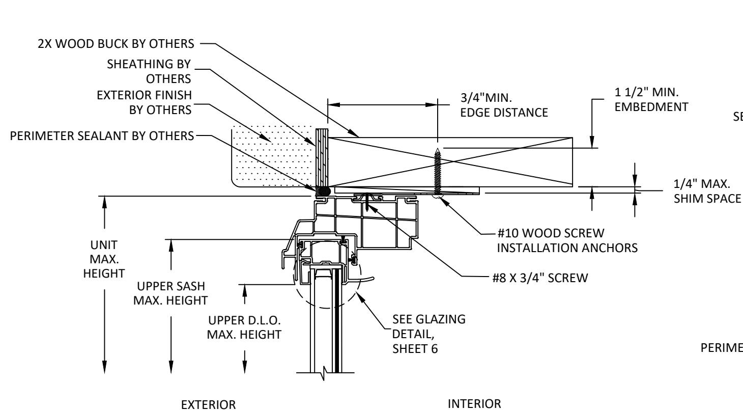
A 5 VERTICAL SECTION CLIP INSTALLATION WOOD BUCK
