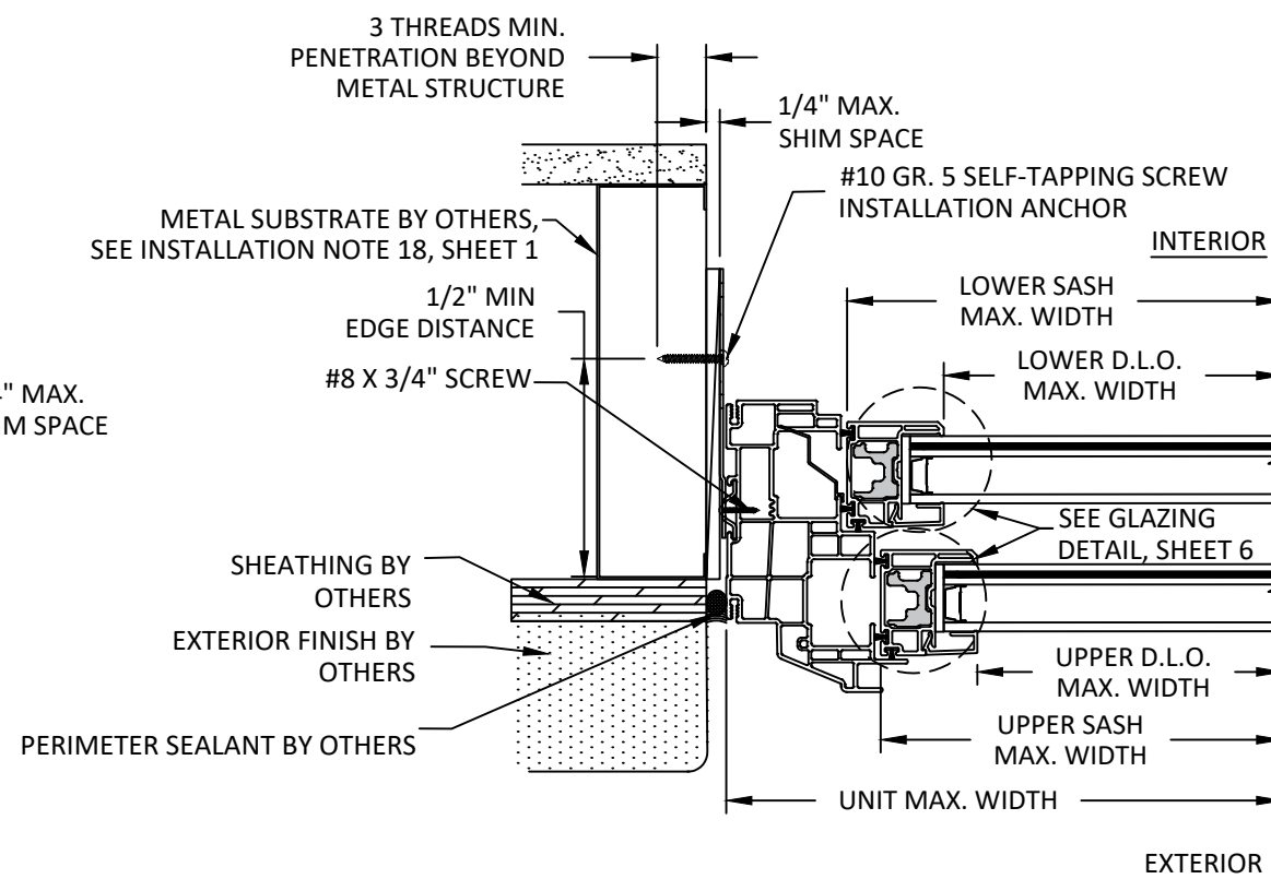
B 5 HORIZONTAL SECTION CLIP INSTALLATION METAL STUD
