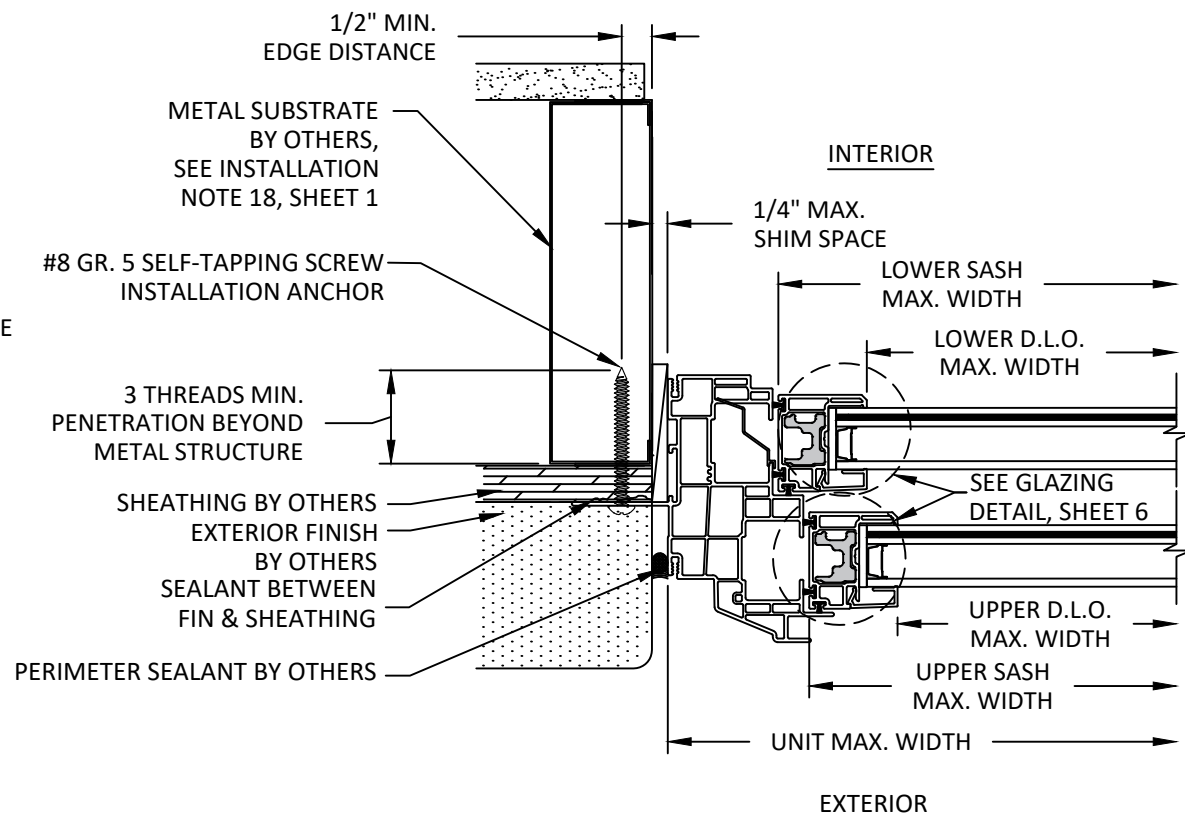
B 3 HORIZONTAL SECTION NAIL FIN INSTALLATION METAL STUD
