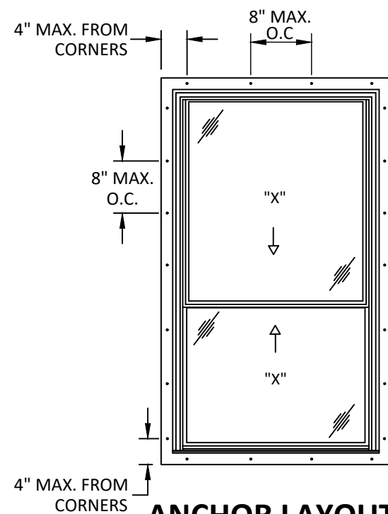
ANCHOR LAYOUT NAILFIN INSTALLATION (EQUAL OR ORIEL)
