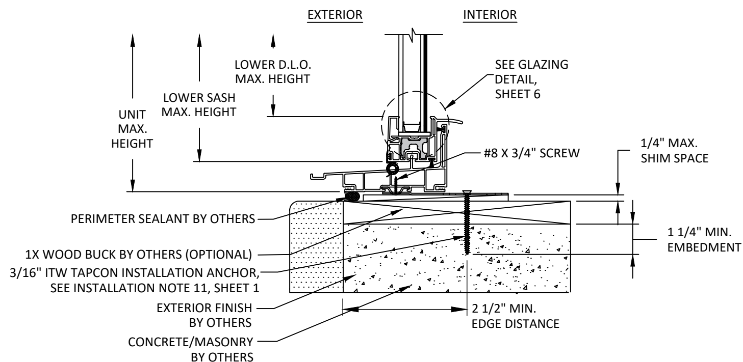
C 5 VERTICAL SECTION CLIP INSTALLATION CONCRETE/CMU
