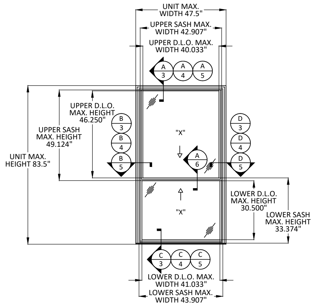
TYPICAL ELEVATION DOUBLE HUNG ORIEL
