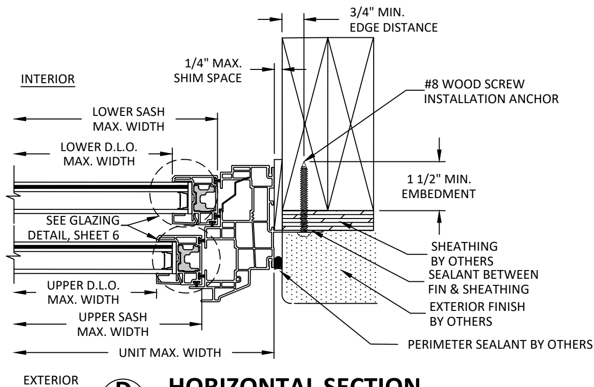
D 3 HORIZONTAL SECTION NAIL FIN INSTALLATION WOOD BUCK
