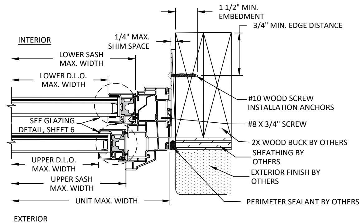
D 5 HORIZONTAL SECTION CLIP INSTALLATION WOOD BUCK
