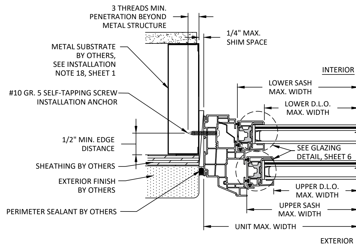
B 4 HORIZONTAL SECTION THROUGH FRAME INSTALLATION METAL STUD
