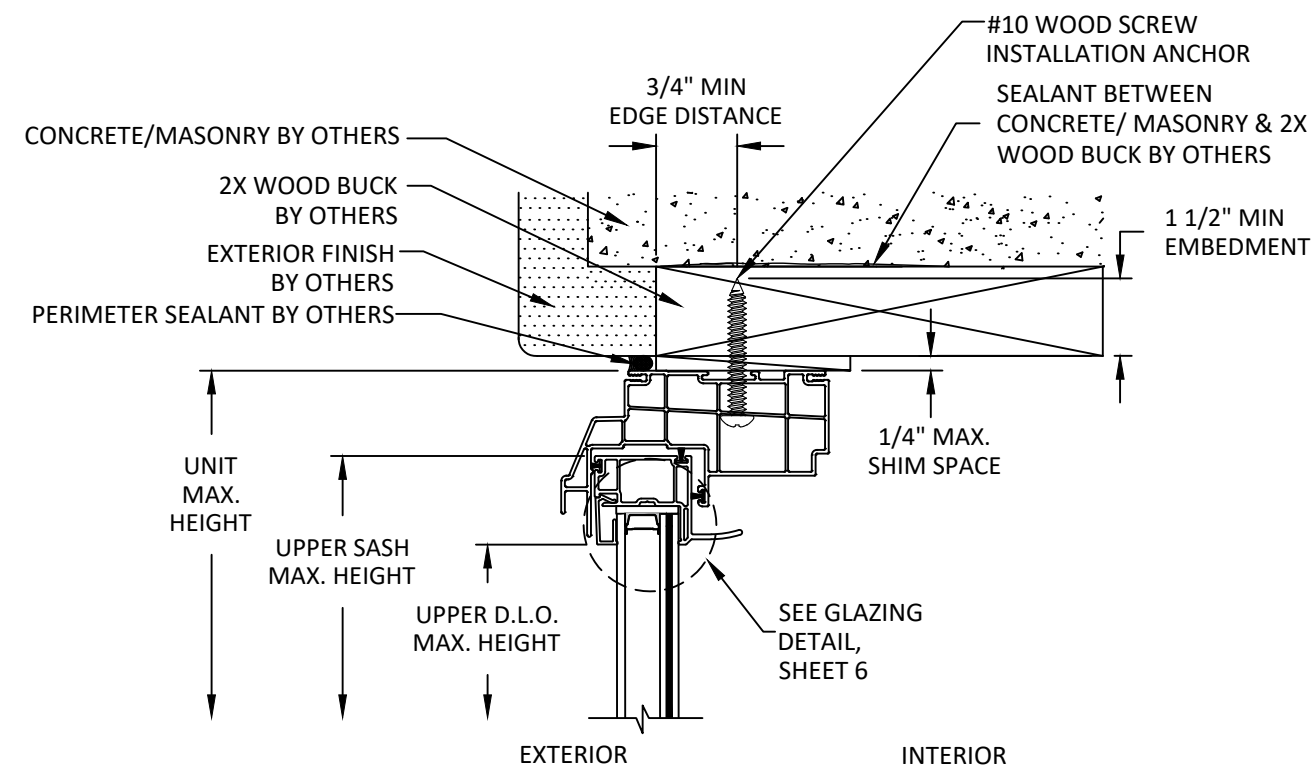
A 4 VERTICAL SECTION THROUGH FRAME INSTALLATION WOOD BUCK
