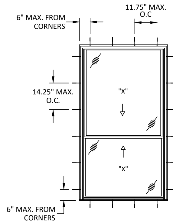
ANCHOR LAYOUT CLIP INSTALLATION (EQUAL OR ORIEL)
